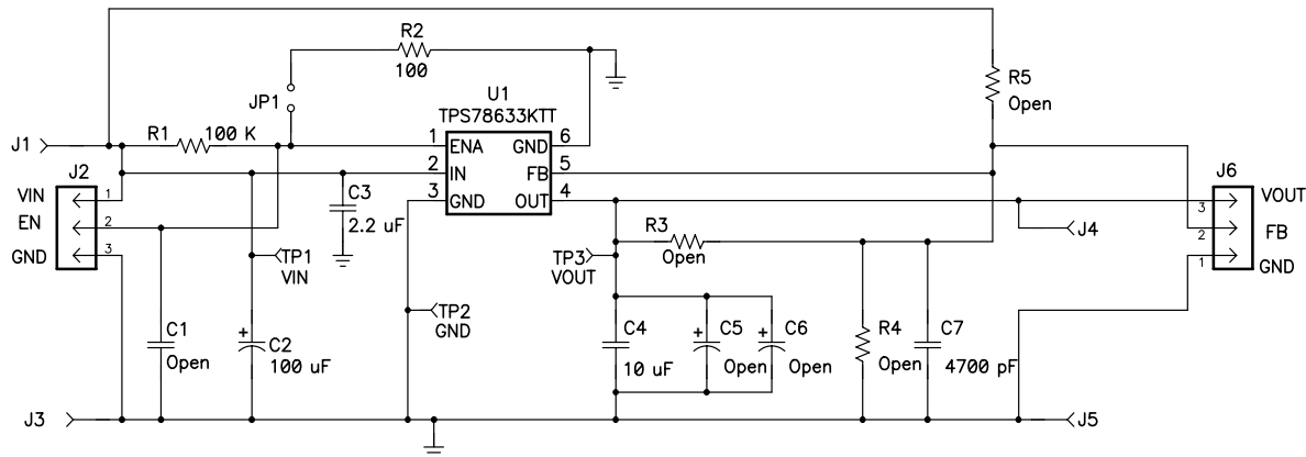
Figure 4–1. Schematic
